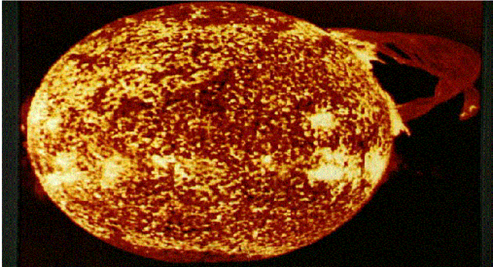
Partial Disruption of Sol (Original Image Credit: NASA, Skylab)
