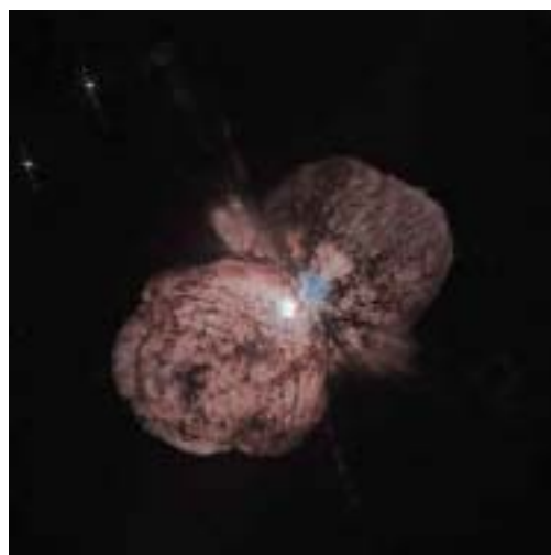
Stellar Explosion (Credit: NASA)
