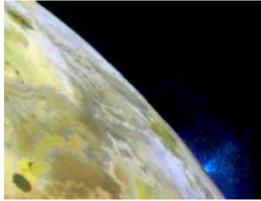
A volcano on Io. Credit: NASA
