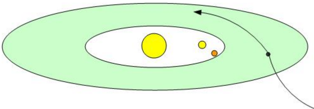
The Accumulation of Mass Selects Angona Planets in the Plane of the Ecliptic
