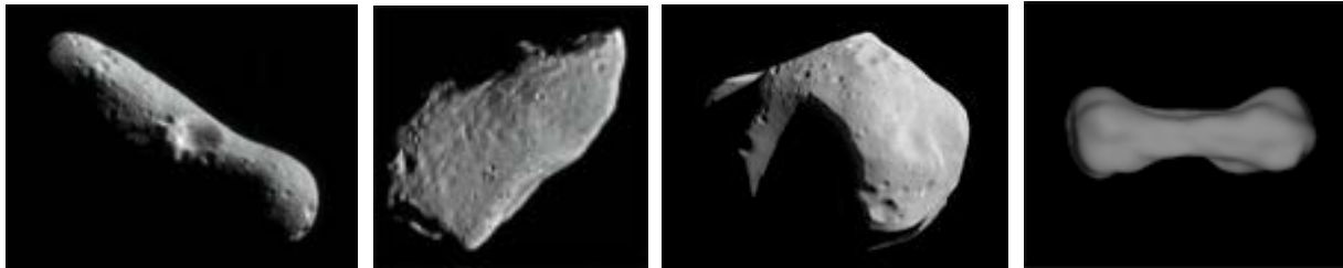
Left to Right: The Asteroids Eros, Gaspra, Mathilde, and Kleopatra Credit: NASA
