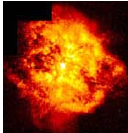
Mechanics of a Supernova Explosion (Credit: NASA)
