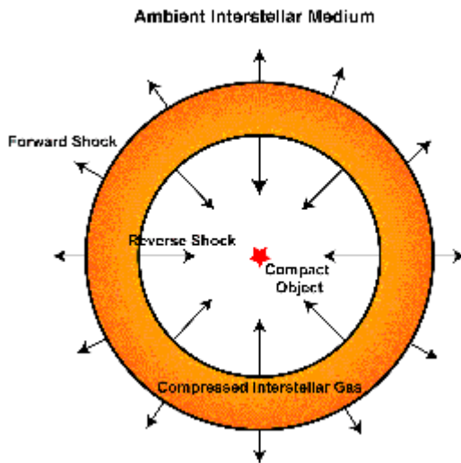
Mechanics of a Supernova Explosion (Credit: NASA)
