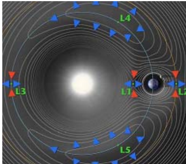
Lagrange Points (Credit: NASA)
