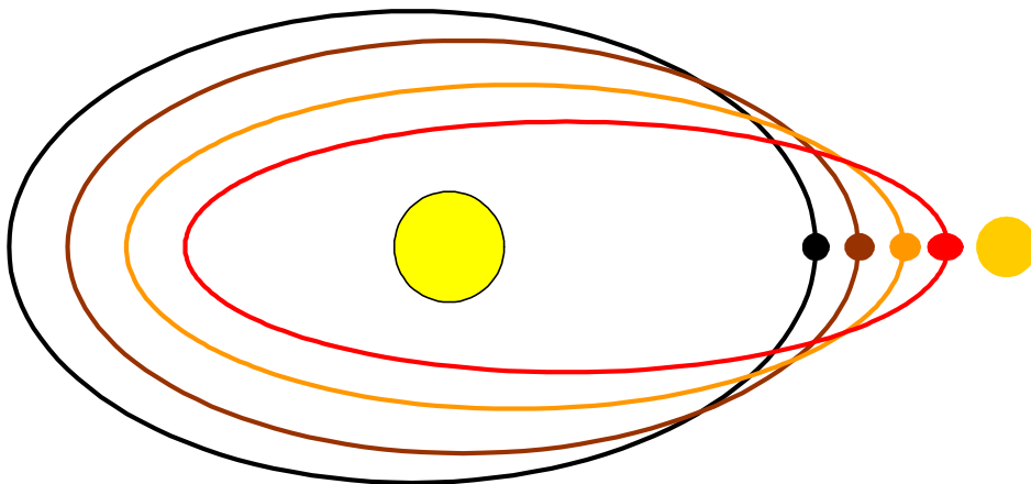
Ceres swings closer and closer to Jupiter over time. (Not to scale.)
