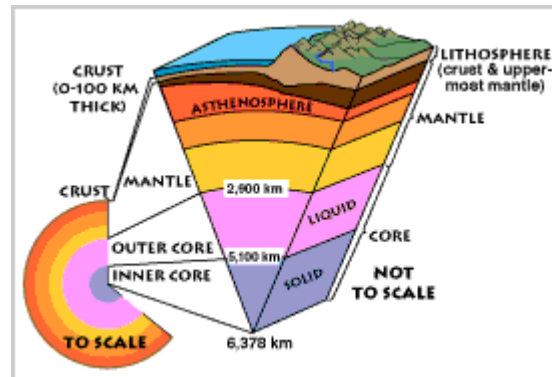
Composition of Earth (Credit: USGS [46])
